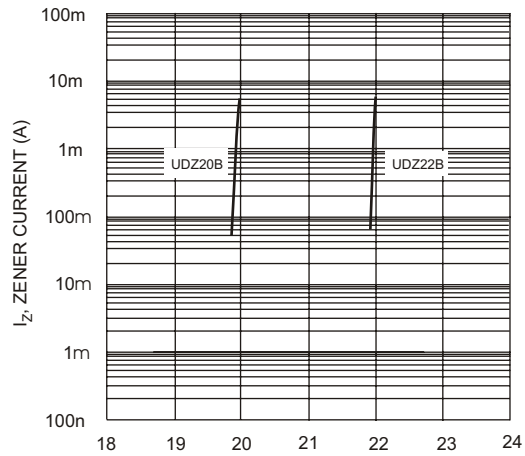
V_Z , ZENER BREAKDOWN VOLTAGE (V) Fig. 5 Typical Reverse Characteristics, UDZ20B - UDZ22B
