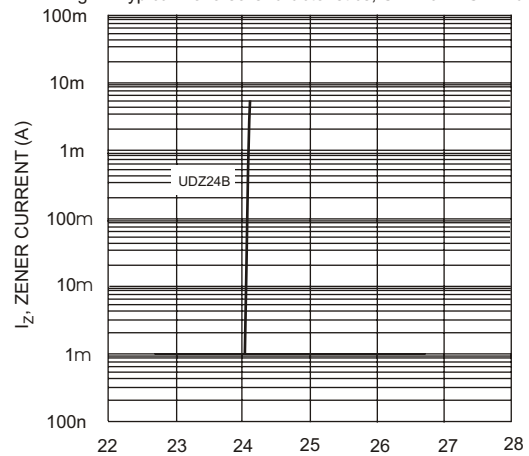
V_Z , ZENER BREAKDOWN VOLTAGE (V) Fig. 6 Typical Reverse Characteristics, UDZ24B
