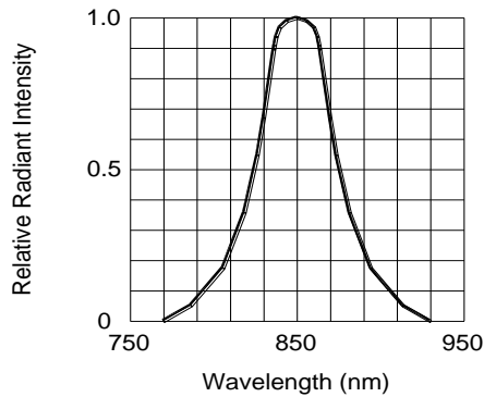
FIG.1 SPECTRAL DISTRIBUTION
