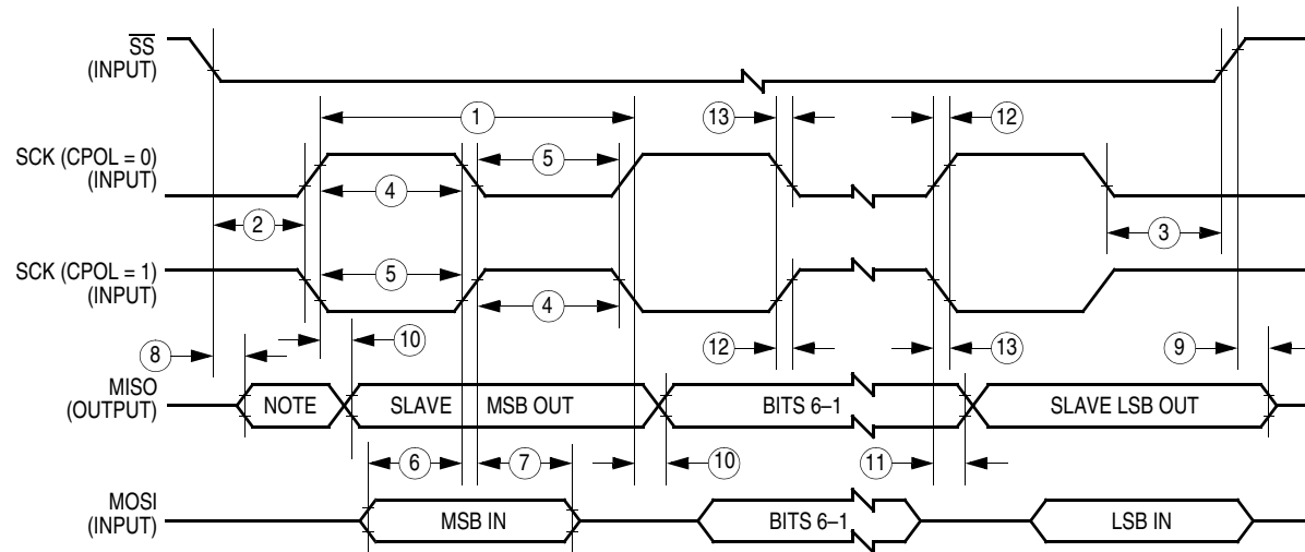
b) SPI Slave Timing (CPHA = 1)
