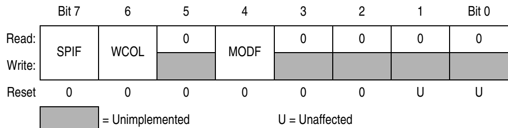
Figure 10-5. SPI Status Register (SPSR)
