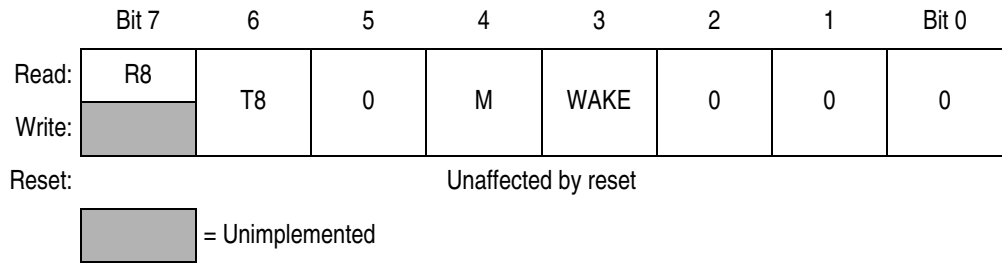
Figure 9-5. SCI Control Register 1 (SCCR1)
