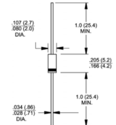
Dimensions in inches and (millimeters) Dimensions in inches and (millimeters)
