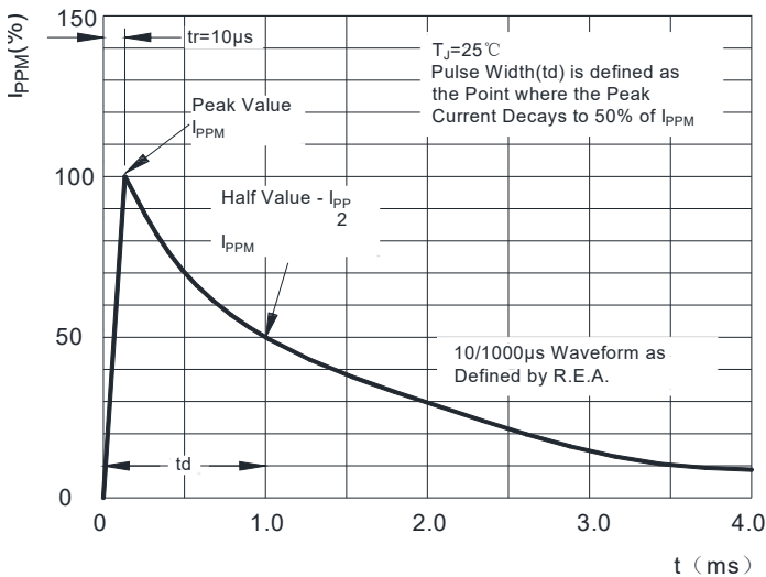
FIG3: Pulse Waveform
