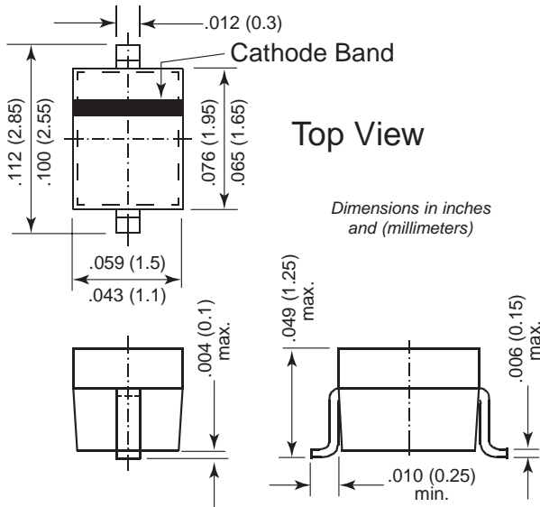
SOD-323
