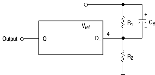
Figure 17. Soft-Start Circuit
