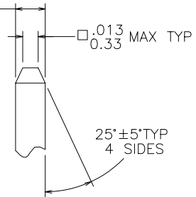
DETAIL P TYP BOTH ENDS
