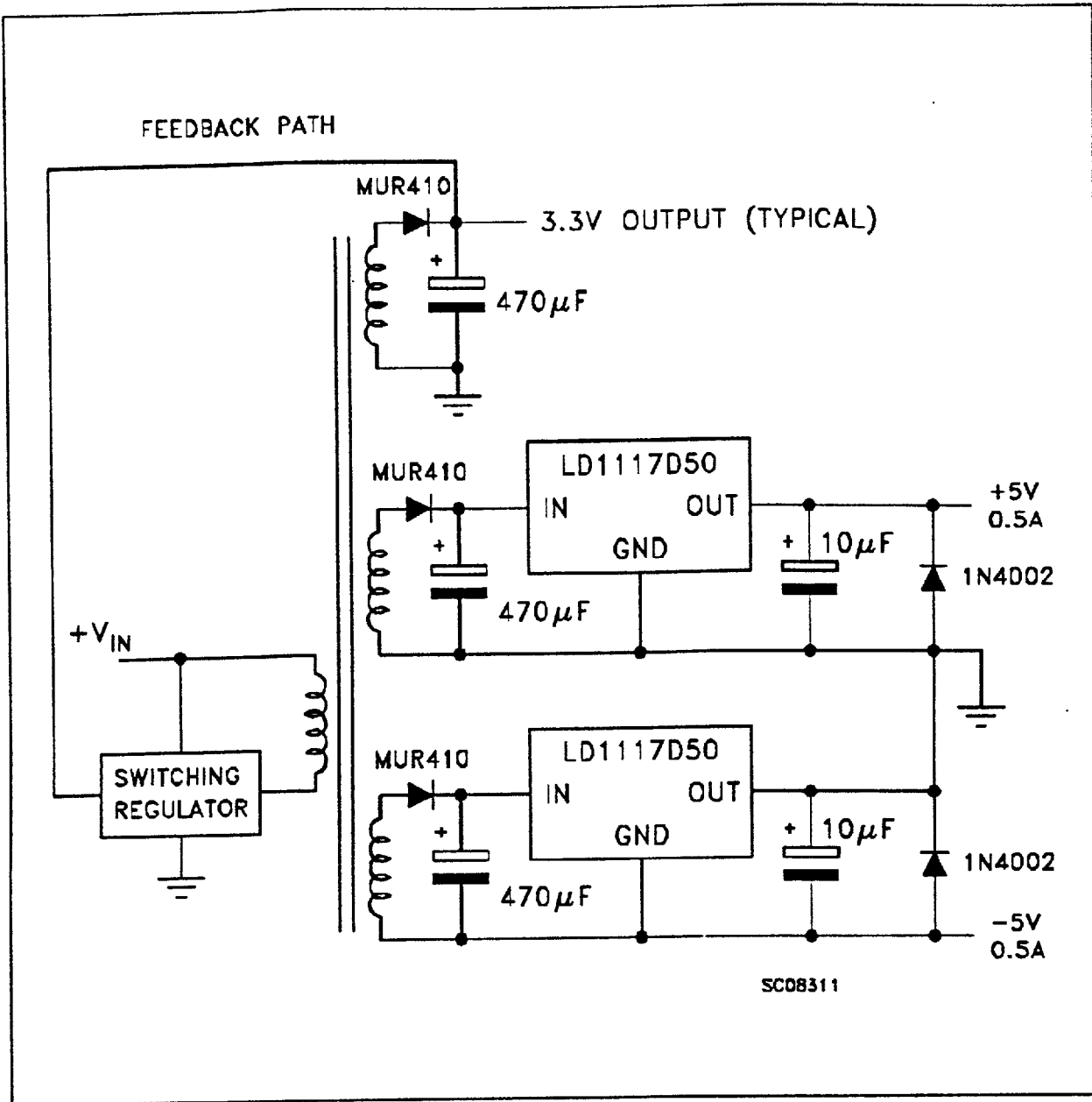
TYPICAL APPLICATIONS (continued): FIGURE 6: Post-Regulated Dual Supply
