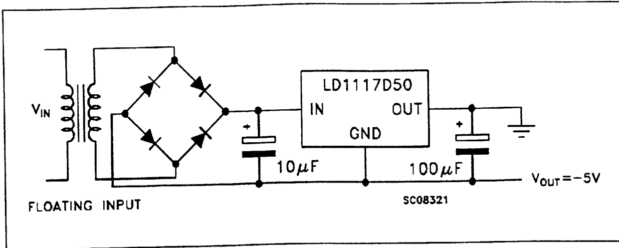
FIGURE 2: Active Terminator for SCSI-2 BUS
