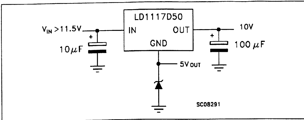
FIGURE 4: Voltage Regulator With Reference
