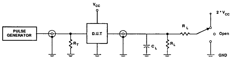
Test Circuit
