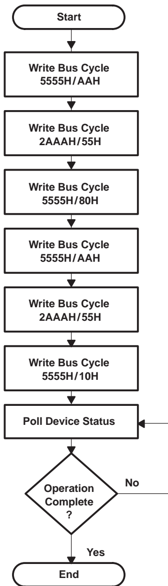
Figure 6. Chip-Erase Algorithm
