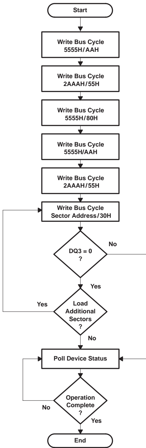
Figure 8. Sector-Erase Algorithm
