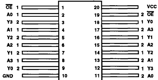
20 PIN CERAMIC FLAT PACK MIL-STD-1835 DESIGNATOR CDFP4-F20, LEAD FINISH C TOP VIEW
