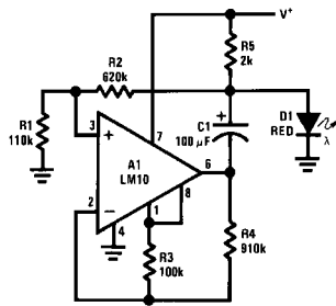
Single-cell Voltage Monitor
