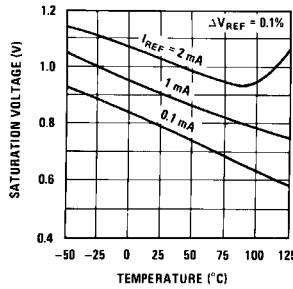
Output Saturation
