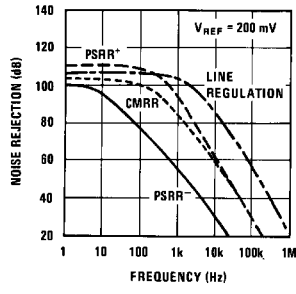
Noise Rejection
