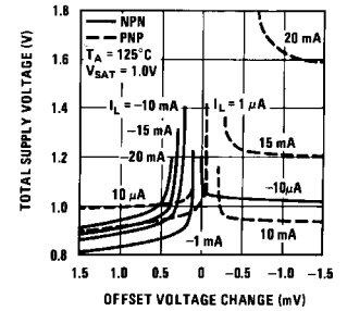
Minimum Supply Voltage
