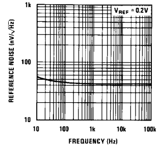
Reference Noise Voltage
