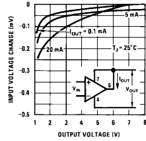
Shunt Gain
