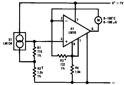
Thermometer
