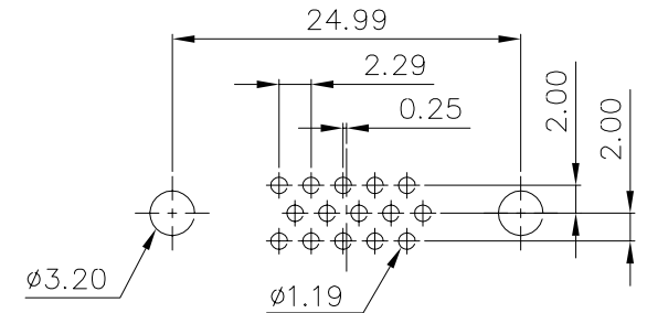
RECOMMEND P.C. BOARD LAYOUT
