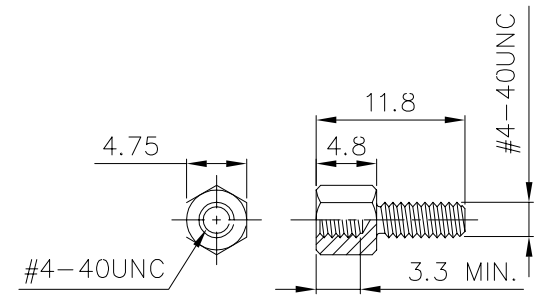
LOCKING SCREW
