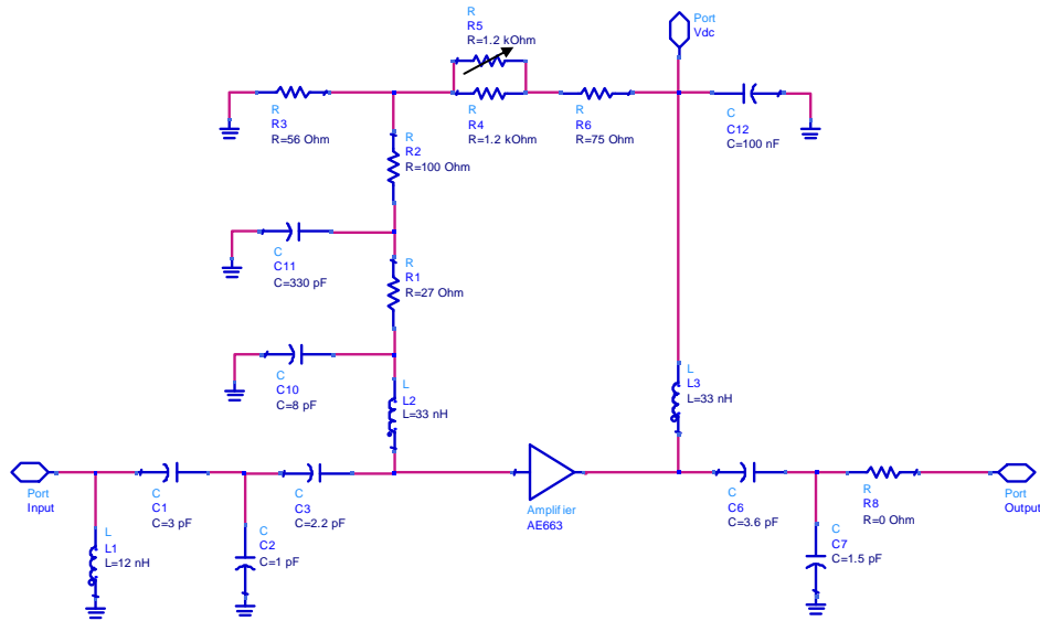
IMT, WCDMA (1920~1980MHz) Performance Data ( V_d=5V, T_c=25^\circ C )
