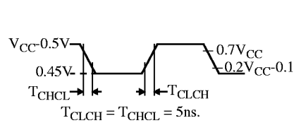
Figure 17. Clock Signal Waveform for I_{CC} Tests in Active and Idle Modes
