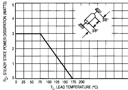
Figure 5. Steady State Power Derating
