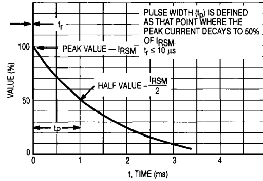
Figure 4. Pulse Waveform
