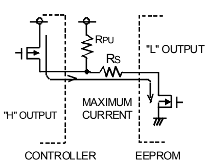
Fig.47 I/O Circuit
