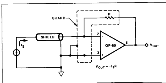
FIGURE 9: Current-to-Voltage Converter
