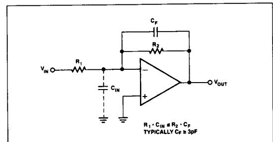
FIGURE 10: Cancelling the Effect of Input Capacitance
