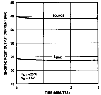
SHORT-CIRCUIT OUTPUT CURRENT vs TIME
