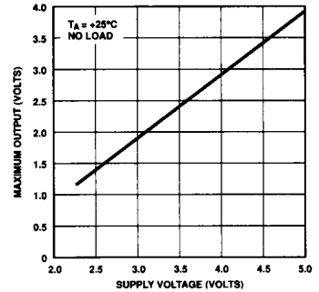
OUTPUT VOLTAGE SWING vs SINGLE SUPPLY VOLTAGE
