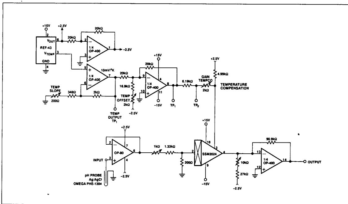
FIGURE 7: A Complete, Temperature-Compensated pH Meter Design
