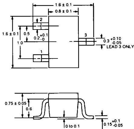
PACKAGE OUTLINE 19
