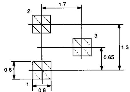
OUTLINE 30 RECOMMENDED P.C.B. LAYOUT
