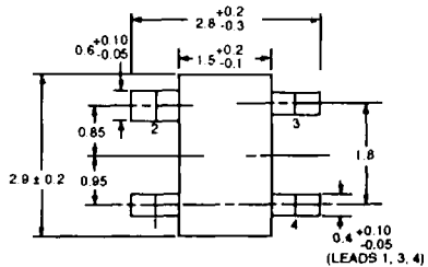
PACKAGE OUTLINE 39 (SOT-143)
