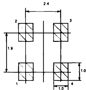
OUTLINE 39 RECOMMENDED P.C.B. LAYOUT
