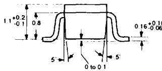
PACKAGE OUTLINE 39 (SOT-143)
