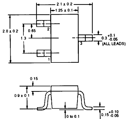
PACKAGE OUTLINE 30 (SOT-323)
