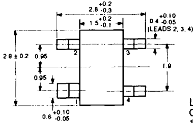
PACKAGE OUTLINE 39 (SOT-143)
