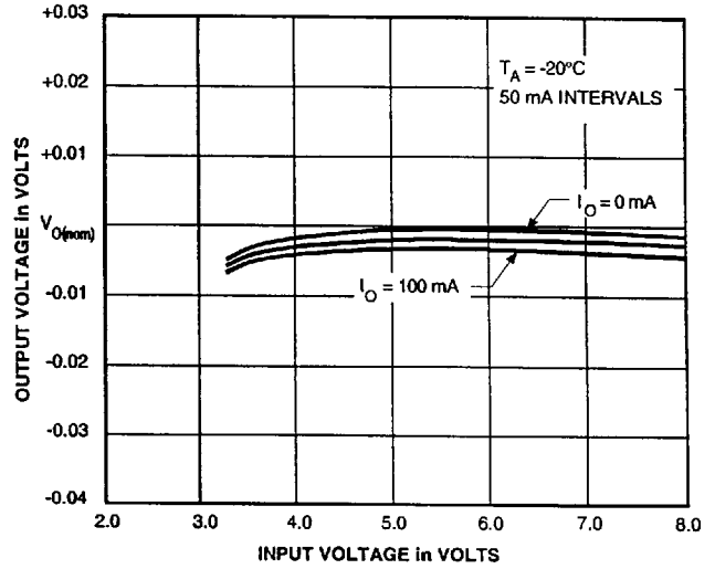
LINE REGULATION
