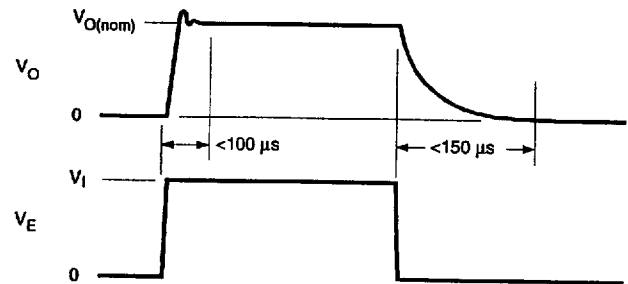
Dwg. WP-027-3
