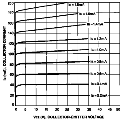
STATIC CHARACTERISTIC
