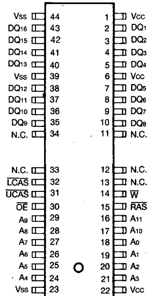
(TSOP(II)-Reverse)
