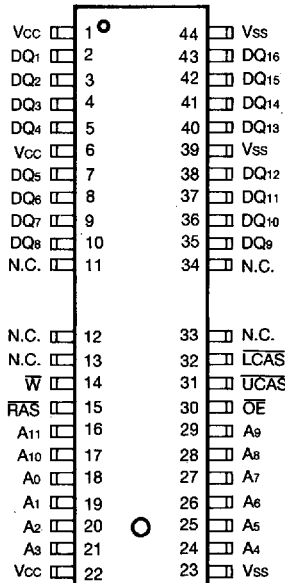
(TSOP(II)-Forward)
