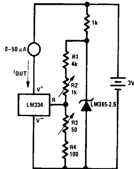
0°F–50°F Thermometer
