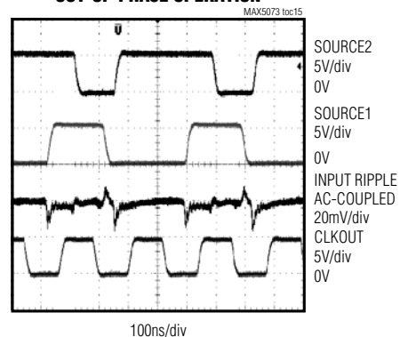
OUT-OF-PHASE OPERATION
