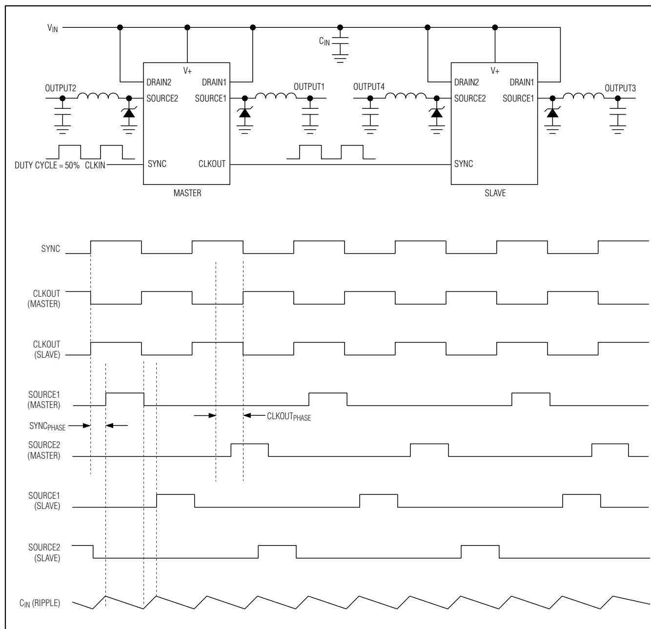
Figure 3. Synchronized Controllers
