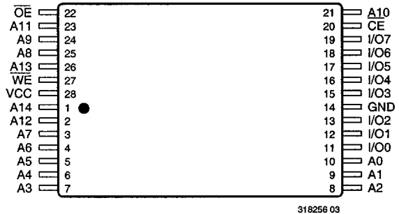
28-Pin TSOP (Reverse)
