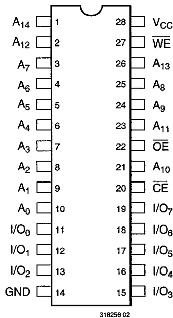
28-Pin DIP/SOP
