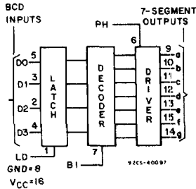
FUNCTIONAL DIAGRAM
