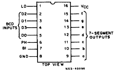
TERMINAL ASSIGNMENT
