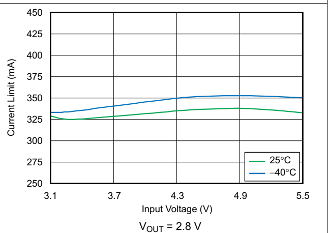
Figure 6-30. Current Limit vs Input Voltage
