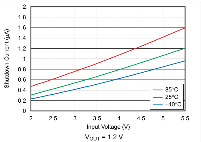
Figure 6-26. Shutdown Current vs Input Voltage
