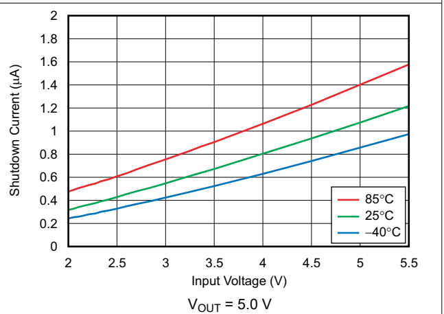
Figure 6-28. Shutdown Current vs Input Voltage
