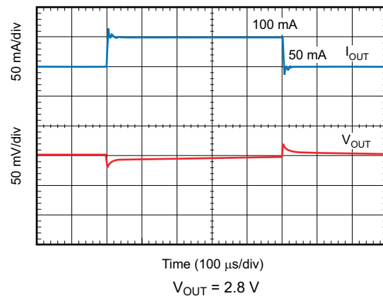
Figure 6-42. Load Transient Response
