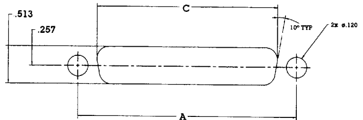
RECOMMENDED PANEL CUTOFF DIMENSIONS
