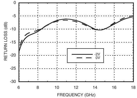
Output Return Loss @ Voltage Extreme
