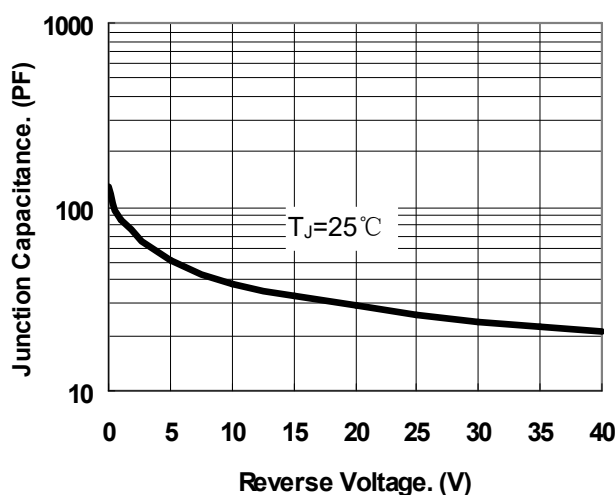
Fig.1-Typical Junction Capacitance
