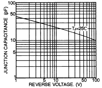
FIG.4-TYPICAL JUNCTION CAPACITANCE
