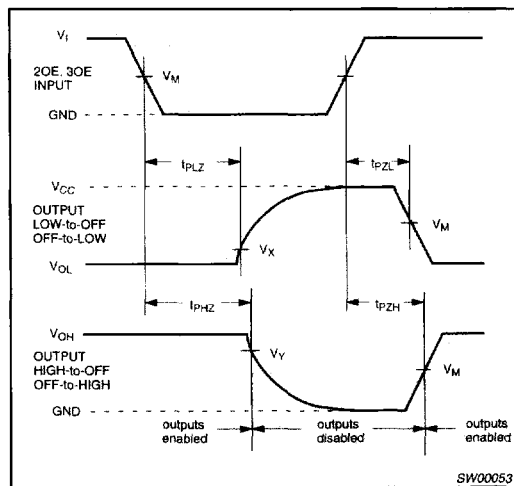
Waveform 2. 3-State enable and disable times for the input (20E, 30E)
