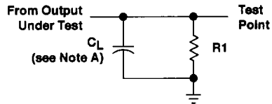
LOAD CIRCUIT FOR TOTEM-POLE OUTPUTS
