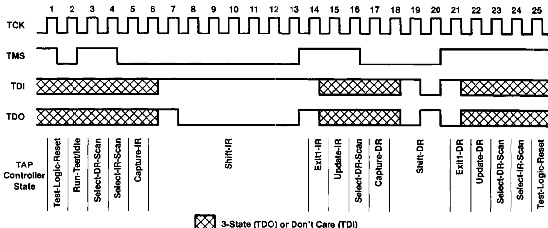
Figure 8. Timing Example
