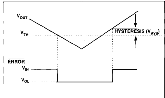
Figure 2. \overline{ERROR} Output Operation
