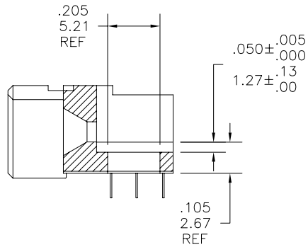
SECTION U-U
