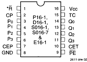
DIP/SOIC/QSOP/CERPACK TOP VIEW
