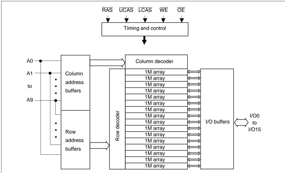
Block Diagram (HM51W18160 Series)
