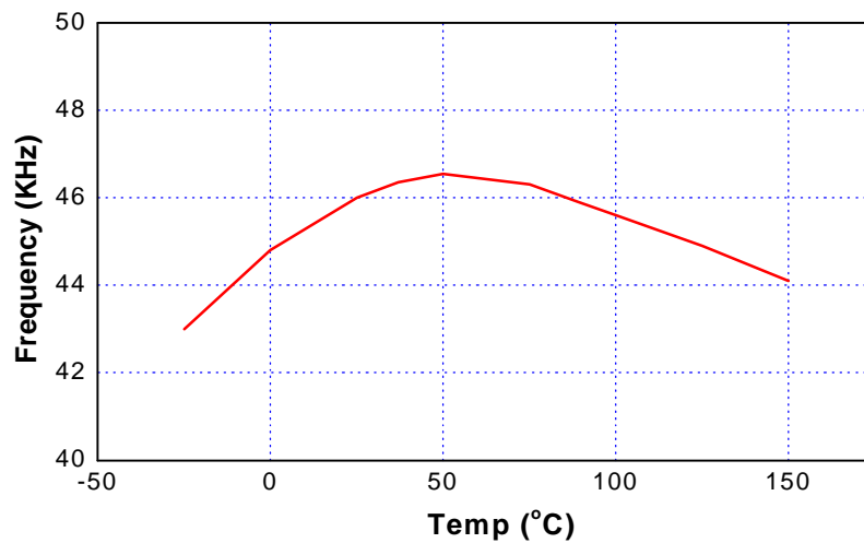
Operating Frequency vs. Temperature
