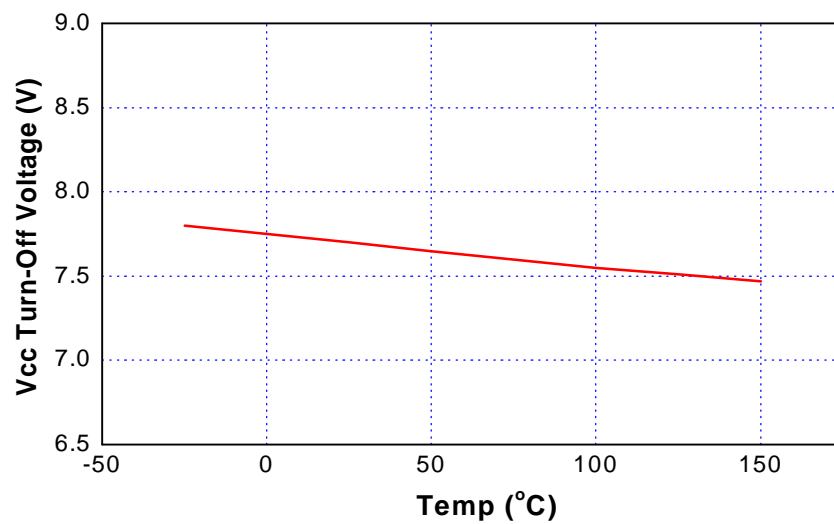
Vcc Turn-Off Voltage vs. Temperature
