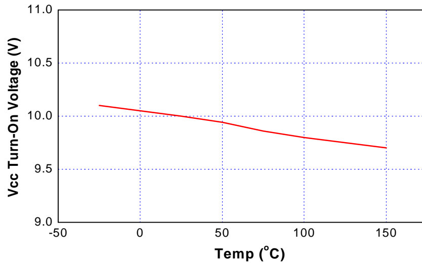
Vcc Turn-On Voltage vs. Temperature
