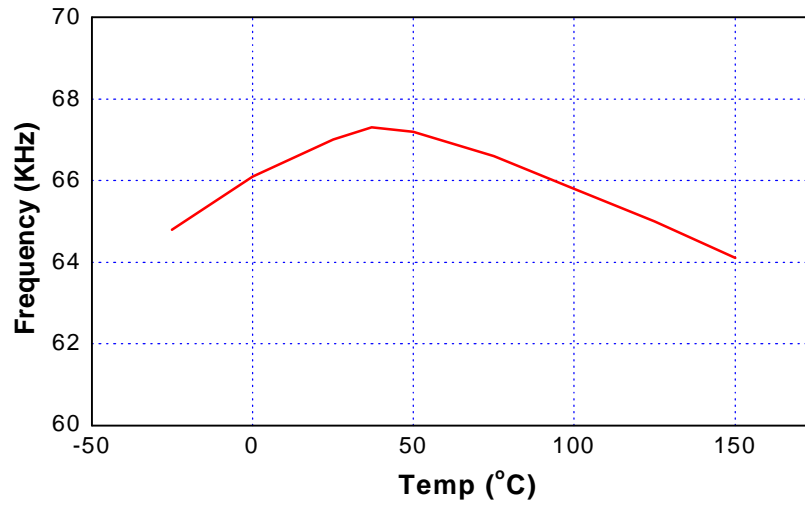
Pre-Heating Frequency vs. Temperature
