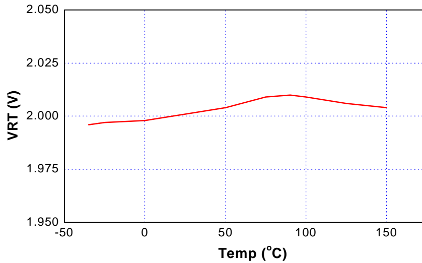
VRT(2.0V) Temperature Stability
