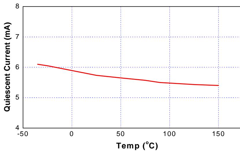
Quiescent Current vs. Temperature
