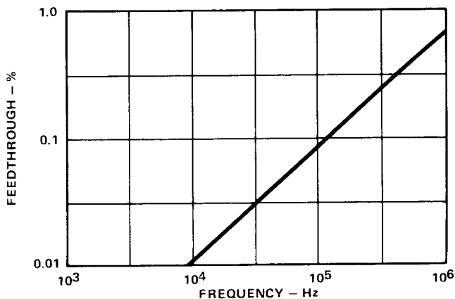
Figure 4. Feedthrough Error vs. Frequency
