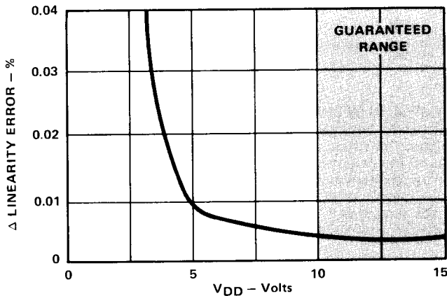
Figure 3. Linearity Error vs. Supply Voltage Typ.
