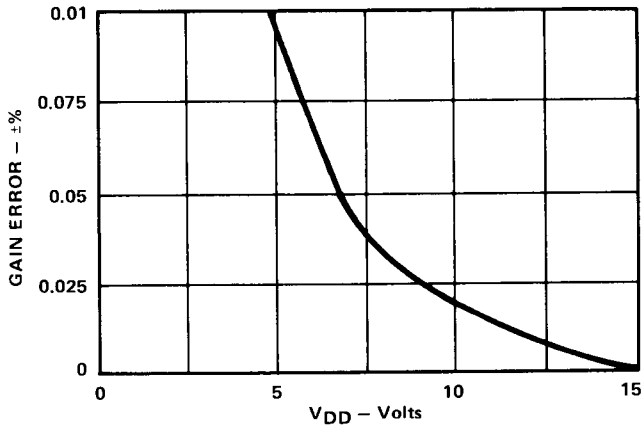
Figure 1. Gain Error vs. Supply Voltage
