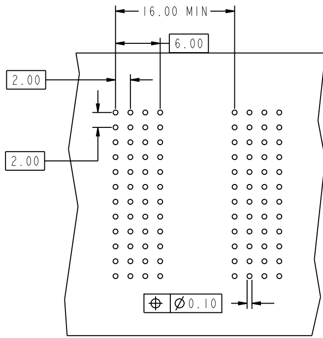
REQUIRED PCB BOARD LAYOUT COMPONENT SIDE
