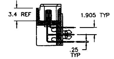
SECTION X-X
