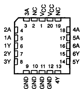
54ACT11004 ... FK PACKAGE
