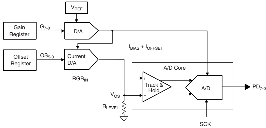
Figure 2. A/D Converter Architecture
