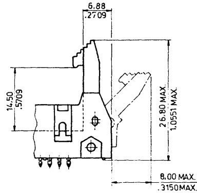
STANDARD LATCH
