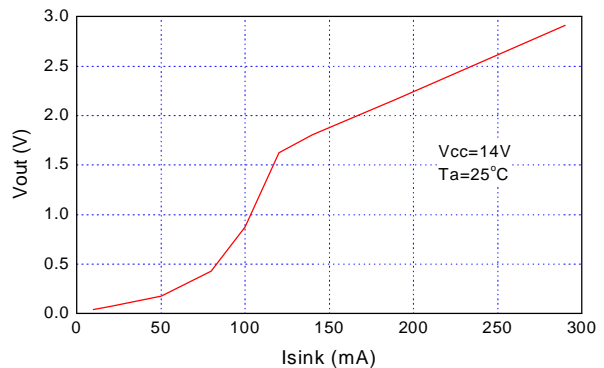
Output Low Voltage
