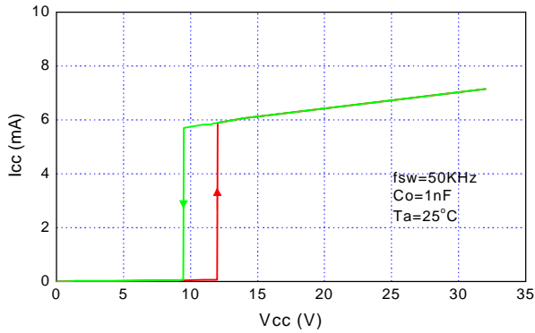
Operating Supply Current
