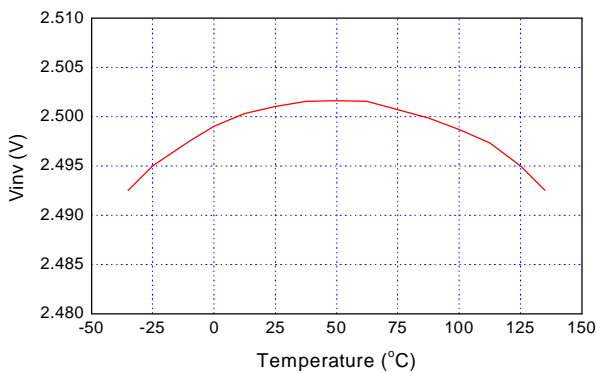
Voltage Feedback Input vs. Temperature
