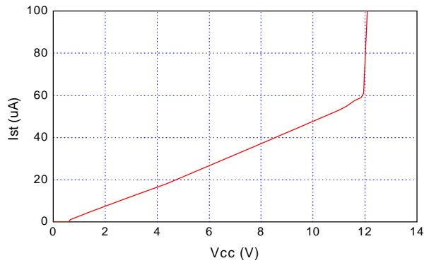
Vcc Start-up Current
