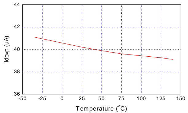
Dynamic OVP Current vs. Temperature
