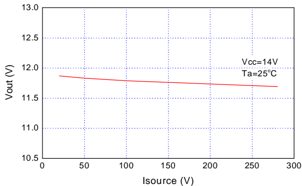
Output High Voltage
