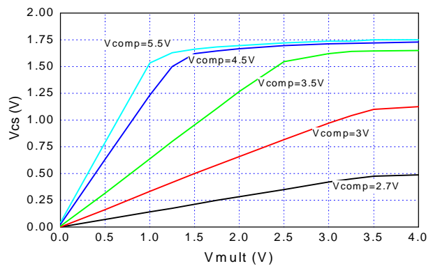
Multiplier Input vs. CS Threshold Voltage
