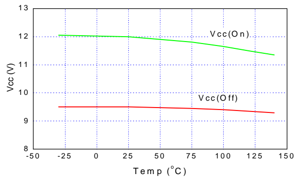
UVLO On/Off Voltage vs. Temp
