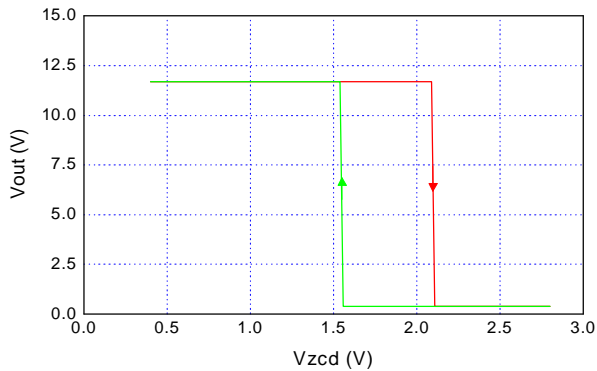
ZCD Input Threshold Voltage
