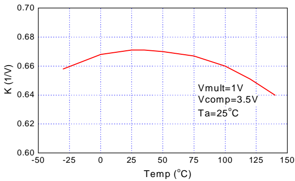
Multiplier Gain vs. Temperature
