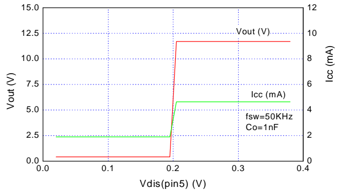
Disable Input Threshold Voltage
