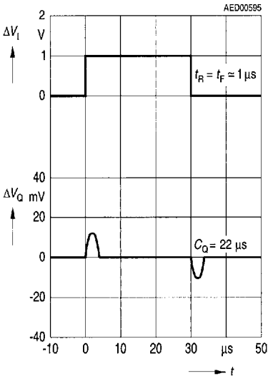
Input Step Response
