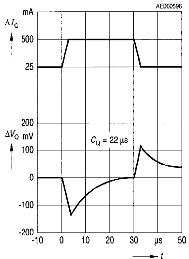
Load Step Response
