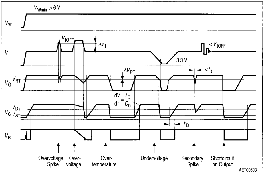
Timing with Watchdog OFF
