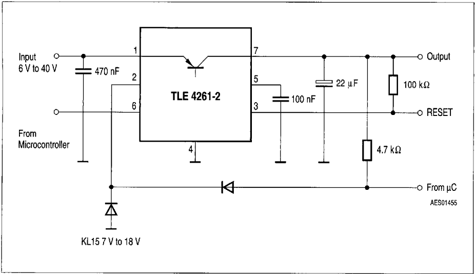
Application Circuit
