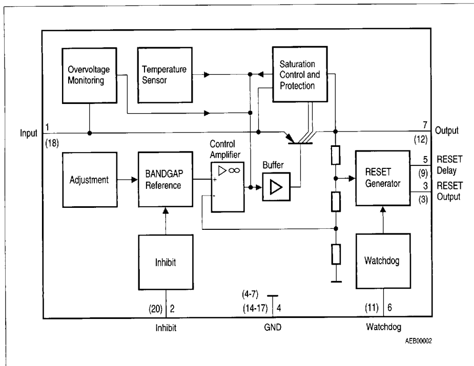
Block Diagram
