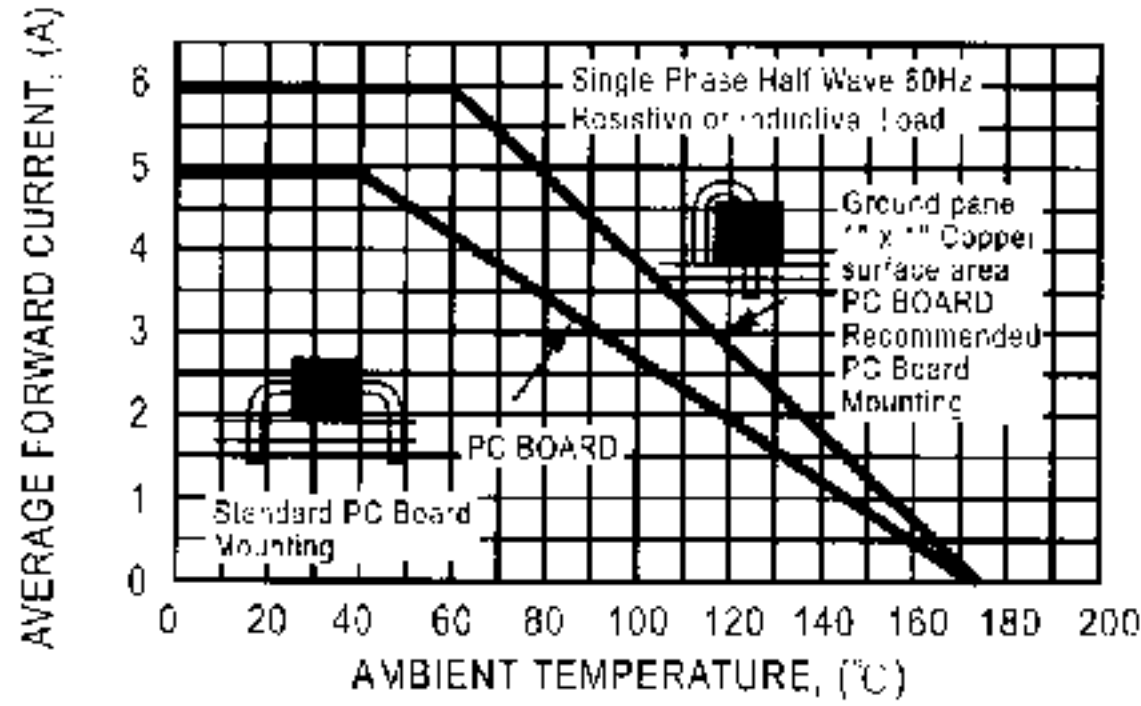
FIG. 1 - TYPICAL FORWARD CURRENT DERATING CURVE
