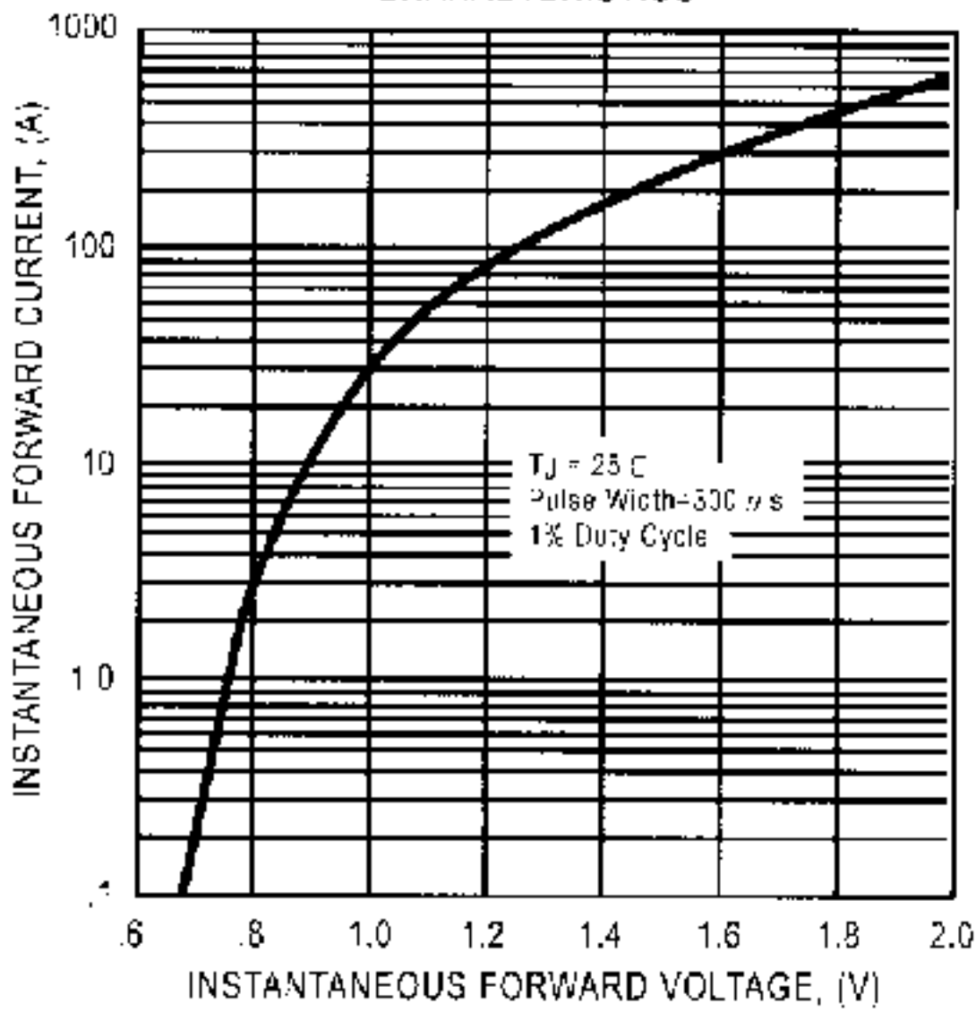
FIG. 2 - TYPICAL INSTANTANEOUS FORWARD CHARACTERISTICS
