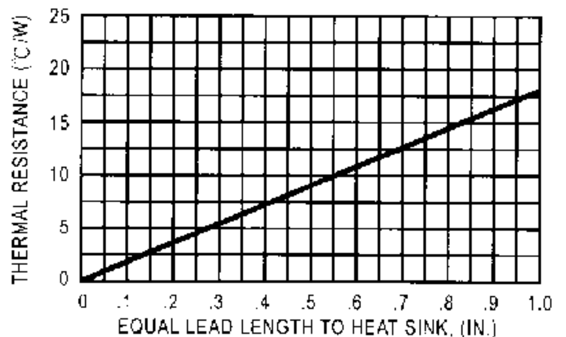
FIG. 5 - TYPICAL THERMAL RESISTANCE VS LEAD LENGTH
