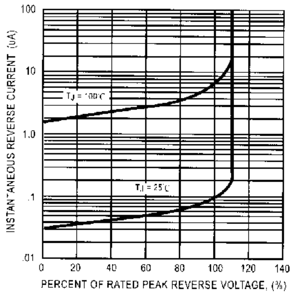
FIG. 3 - TYPICAL REVERSE CHARACTERISTICS
