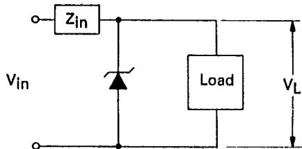
TYPICAL PROTECTION CIRCUIT
