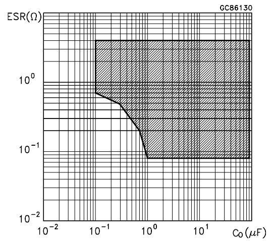
Figure 17 : Stability
