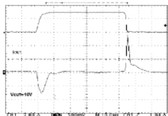
Figure 21 : Load Transient
