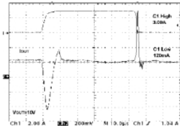
Figure 20 : Load Transient
