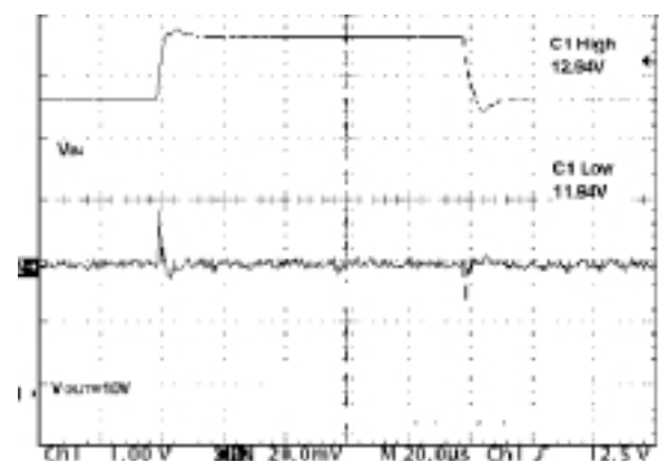
Figure 18 : Line Transient
