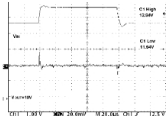
Figure 19 : Line Transient
